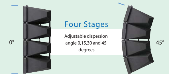
Controlled dispersion
